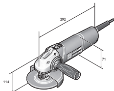
HFW 9-125
