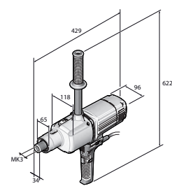
BOZ 32-4 M
