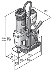
KBM 50 Q
