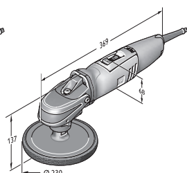
WPO 14-25 E
