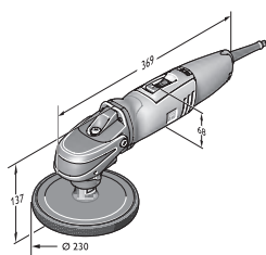
WPO 14-25 E
