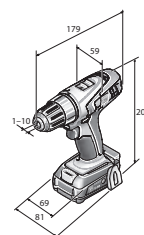
ABSU 12
