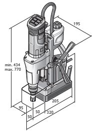
KBM 65 U
