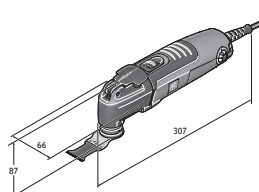
MM 300
