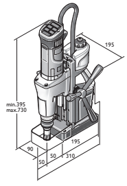
KBM 50 U
