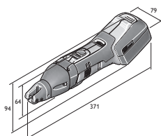
ABSS 18 1.6 E
