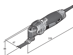
MM 500
